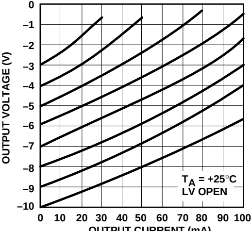
Output Voltage vs. Output Current C_1, C_2 = 1\mu\text{F}
