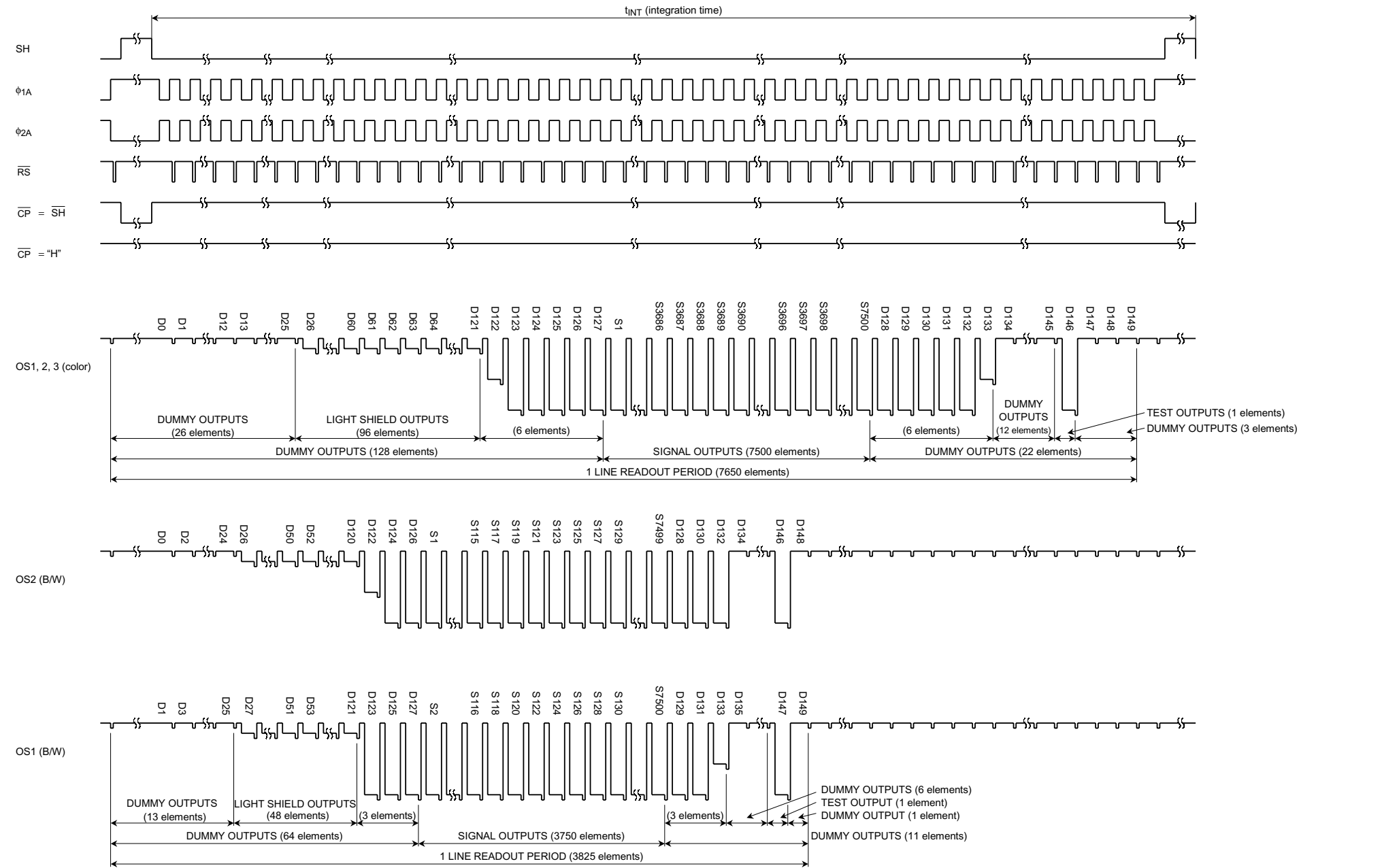
Timing Chart 2: Line Clamp Mode (color or B/W mode)
