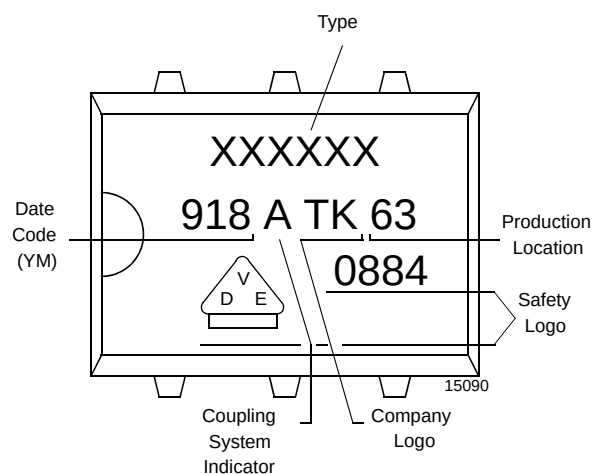
Figure 15. Marking example
