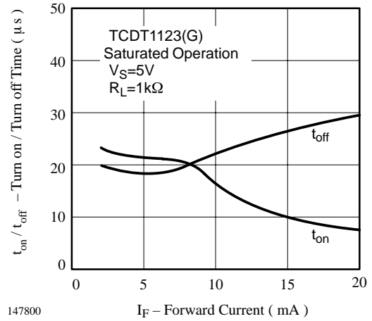
147800 Figure 17. Turn on / off Time vs. Forward Current
