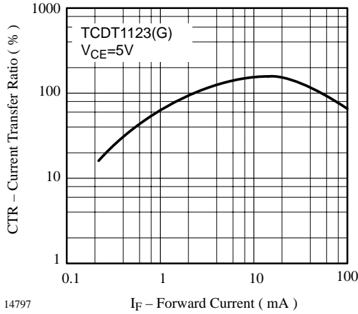
14797 Figure 14. Current Transfer Ratio vs. Forward Current
