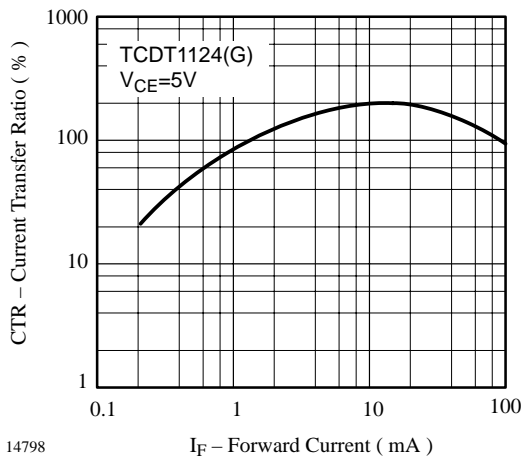
14798 Figure 15. Current Transfer Ratio vs. Forward Current
