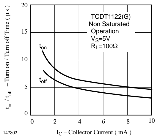
147802 Figure 19. Turn on / off Time vs. Collector Current
