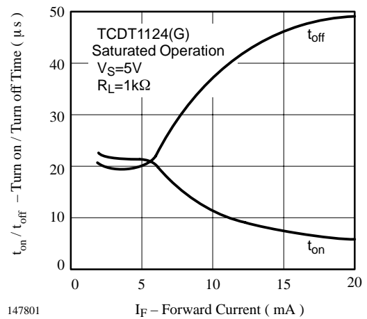
147801 Figure 18. Turn on / off Time vs. Forward Current
