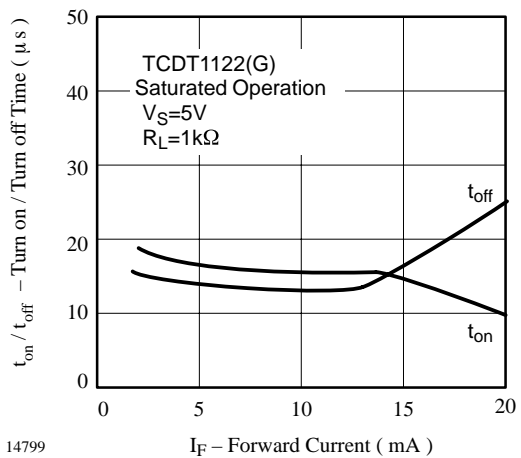
14799 Figure 16. Turn on / off Time vs. Forward Current
