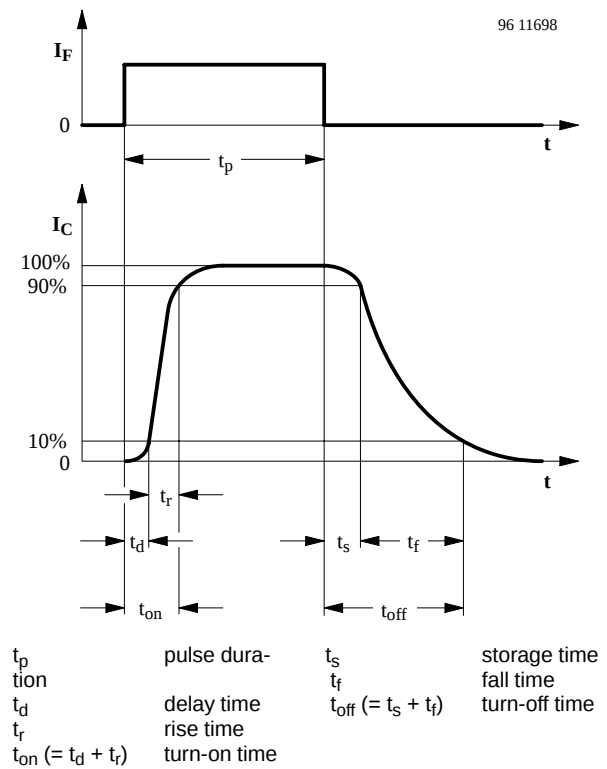
Figure 4. Switching times
