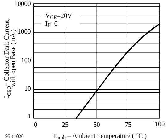
Figure 9. Collector Dark Current vs. Ambient Temperature
