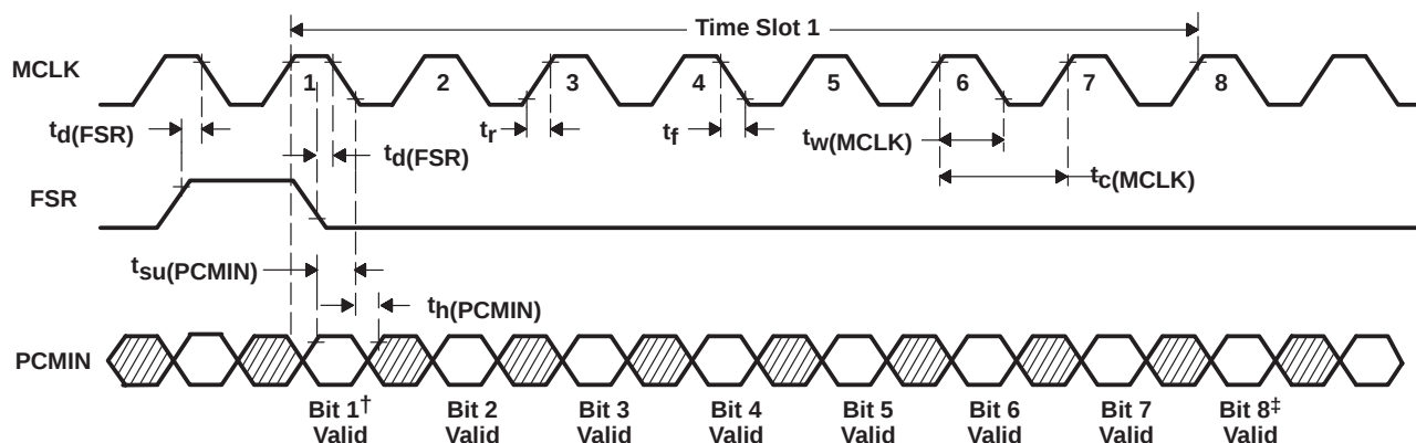
Figure 3. Transmit Timing
