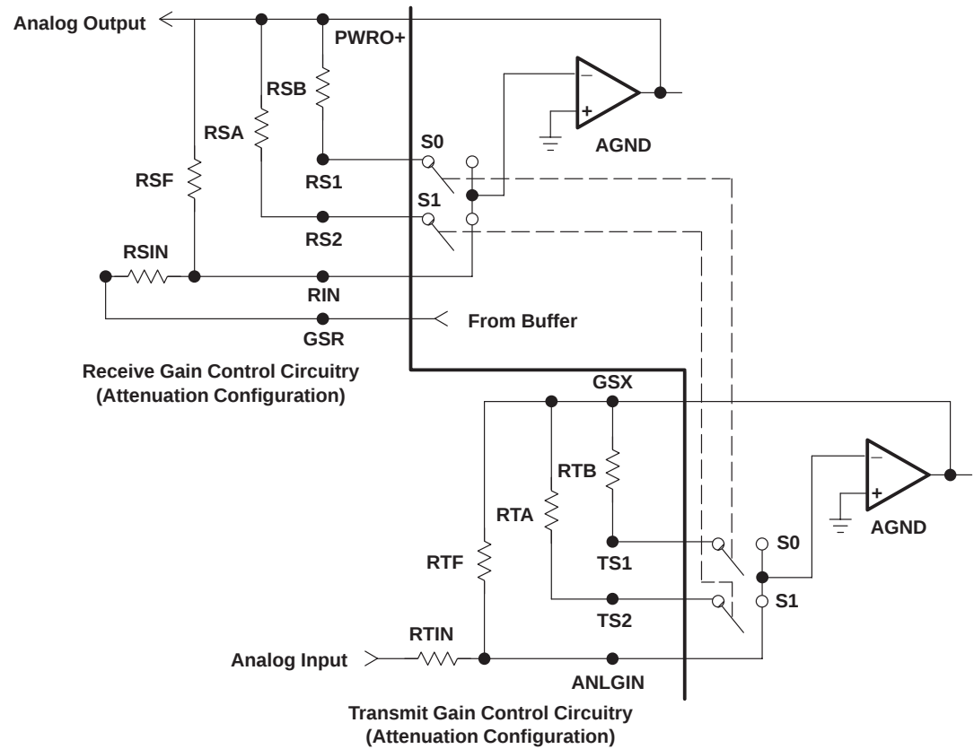
Figure 7. Attenuation Control Circuitry
