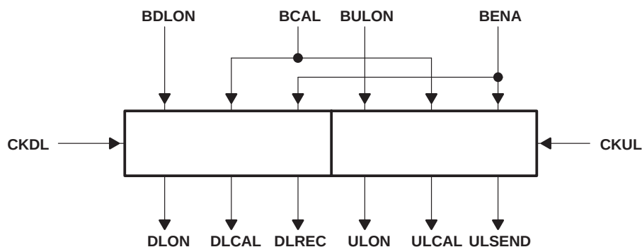
Figure 17. Timing Interface
