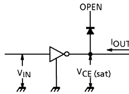
2. V_{CE(sat)}
