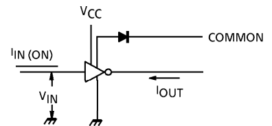
3. I_{IN(ON)}
