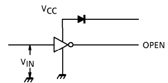
6. I_{CC(ON)}, I_{CC(OFF)}
