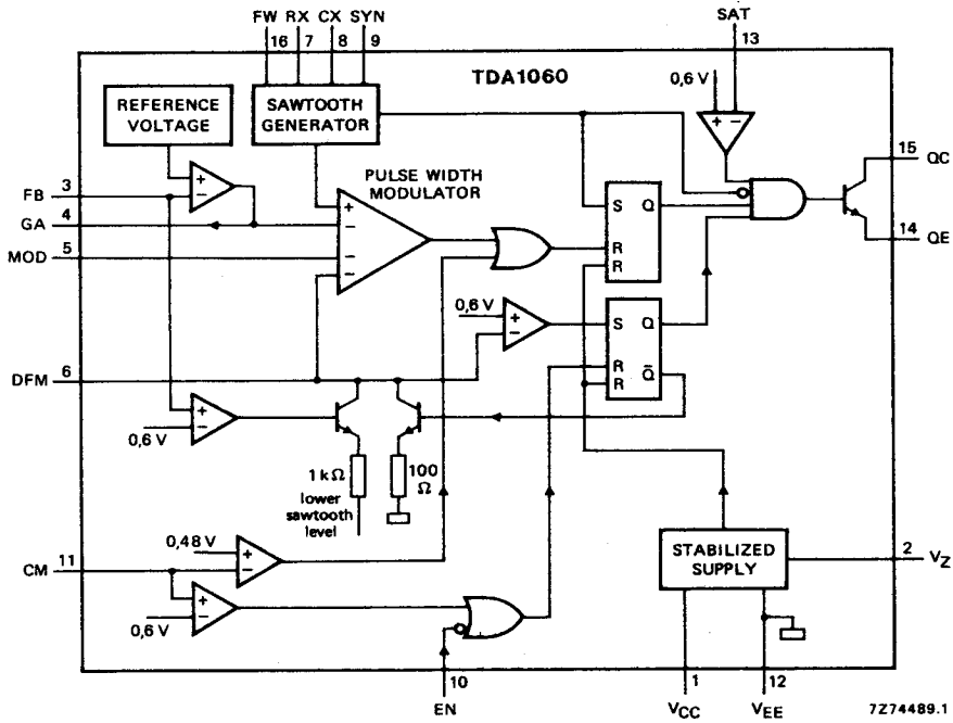
Fig. 1 Block diagram.
