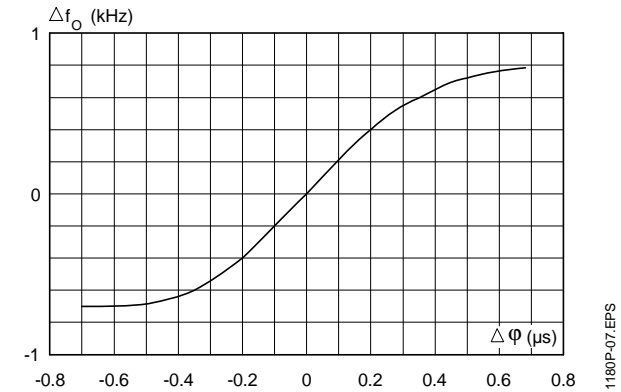
Figure 4 : Loop Gain
