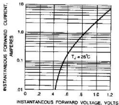
Fig. 1-TYPICAL FORWARD CHARACTERISTICS
