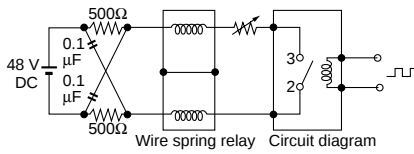
Circuit
