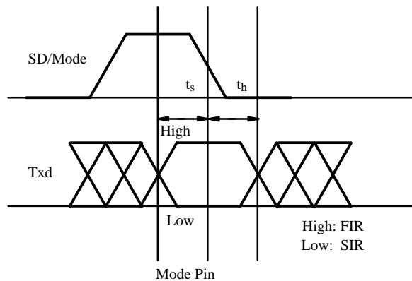
Figure 3. Timing Diagram
