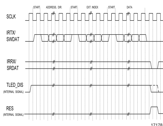
Figure 11. Write Data Waveform with Extended Index
