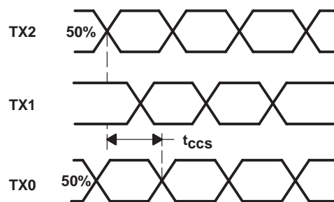
Figure 11. Analog Input Channel-to-Channel Skew
