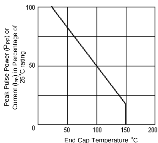
FIGURE 2 Derating Curve
