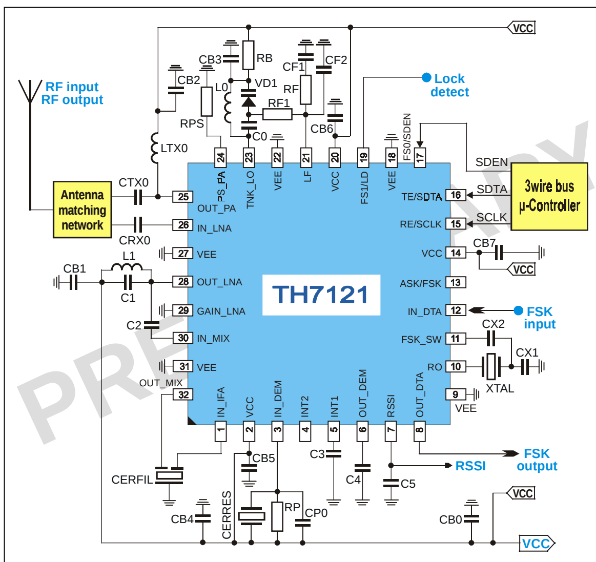
Figure 4: Test circuit for programmable channel FSK operation
