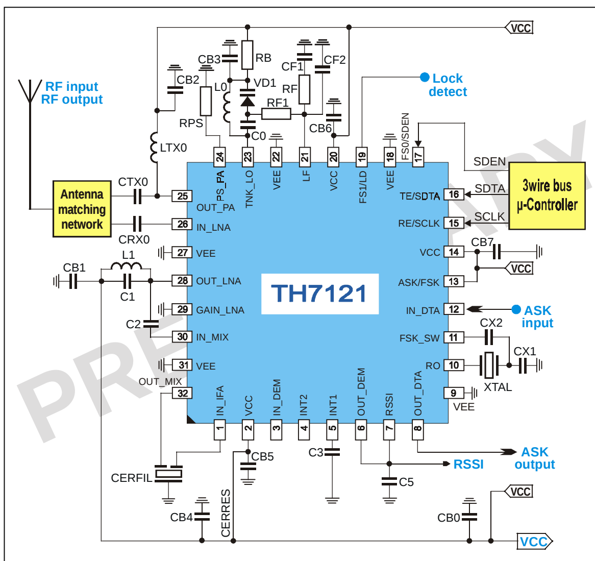
Figure 6: Test circuit for programmable channel ASK operation
