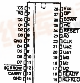
THCT12016NL 28 Pin/600mll
