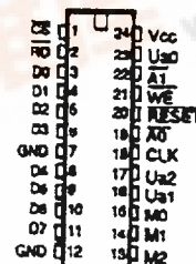
THCT12024NL 24Pin/300mll
