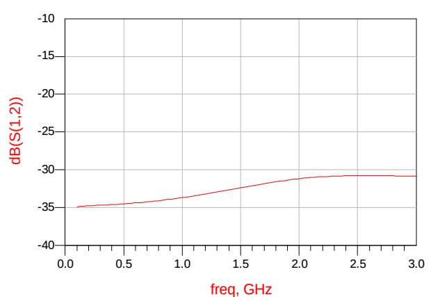
Fig4. Isolation
