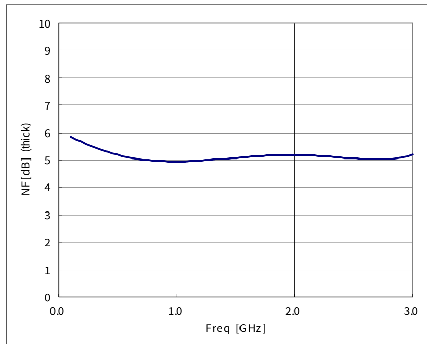
Fig7. Noise Figure
