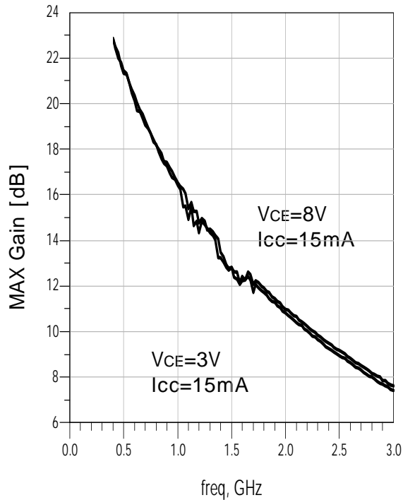
Power Gain : MSG vs. Frequency
