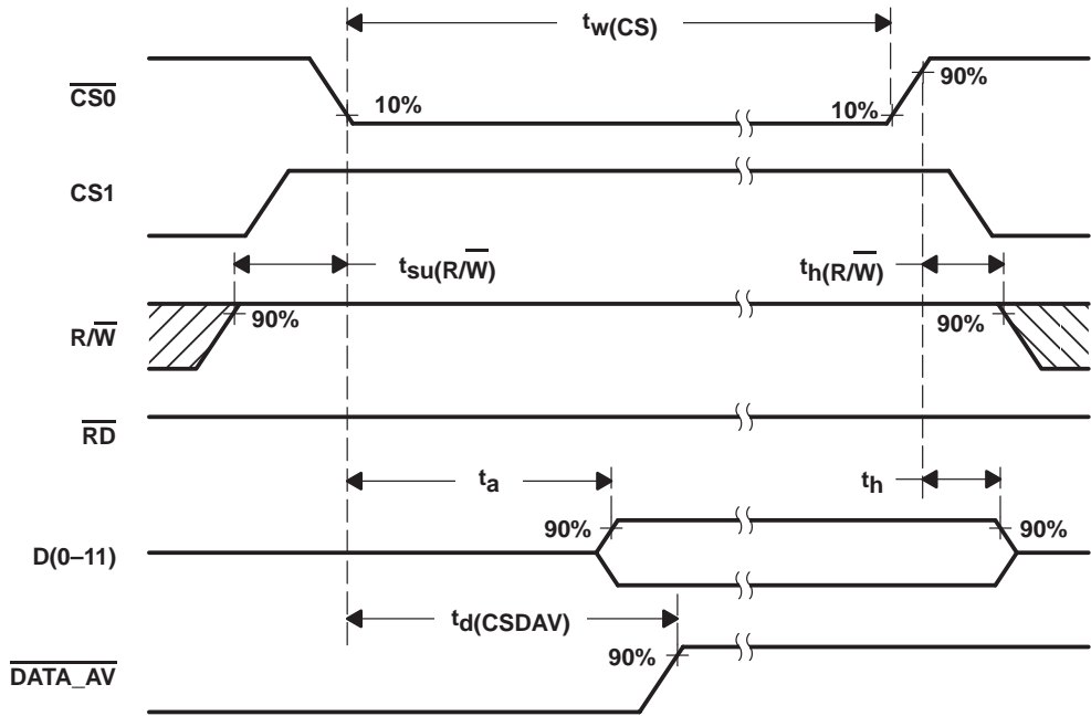
Figure 11. Read Timing Diagram Using \overline{R/\overline{W}} ( \overline{CS0} -controlled)
