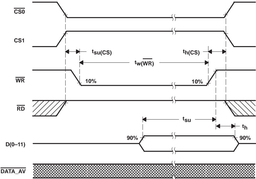
Figure 14. Write Timing Diagram Using \overline{\text{WR}} ( \overline{\text{WR}} -controlled)
