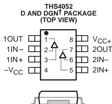
Cross Section View Showing PowerPAD™ Option (DGN)
