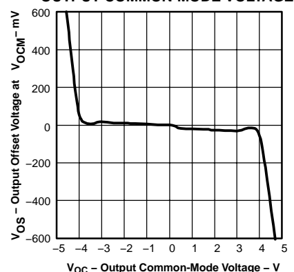
OUTPUT OFFSET VOLTAGE AT V_{OCM} vs OUTPUT COMMON-MODE VOLTAGE
