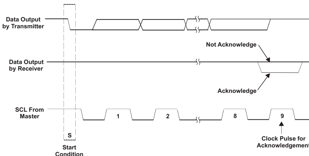
Figure 7. I²C Acknowledge
