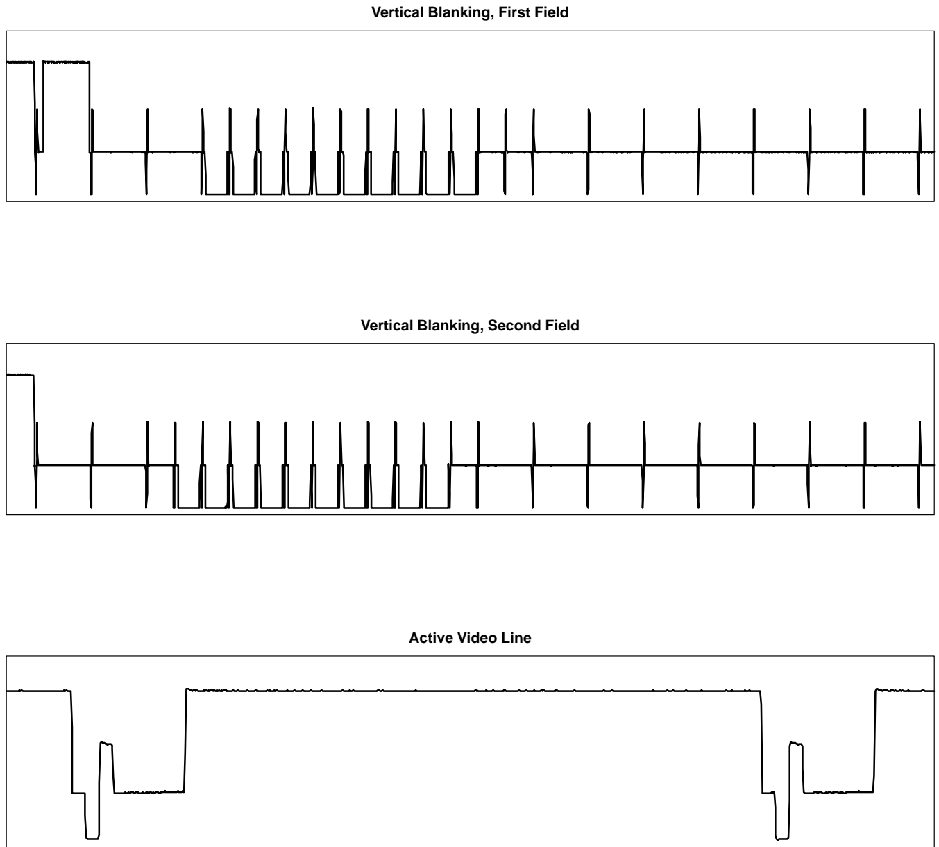
Figure 7-1. THS8200 Output Waveforms for 1080I: Vertical Blanking in First and Second Fields, and Active Video
