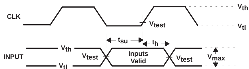
Figure 21. Input Timing Measurement Conditions
