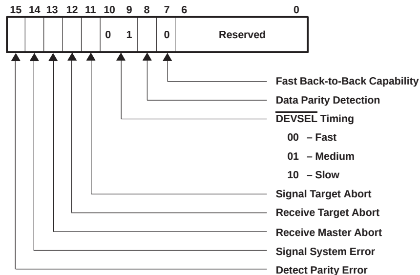
Figure 9. Status Register Layout
