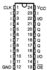
TIBPAL20R6' JT OR NT PACKAGE (TOP VIEW)
