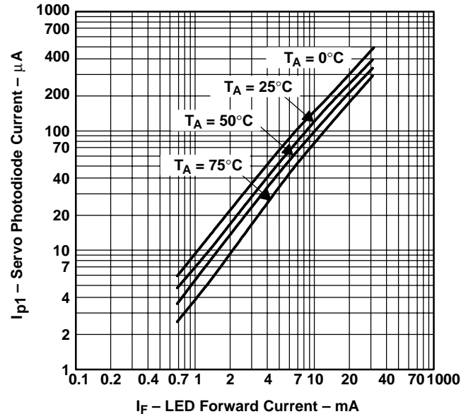
SERVO PHOTODIODE CURRENT vs LED FORWARD CURRENT AND TEMPERATURE
