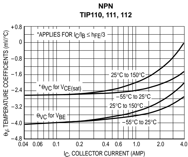
Figure 11. Temperature Coefficients
