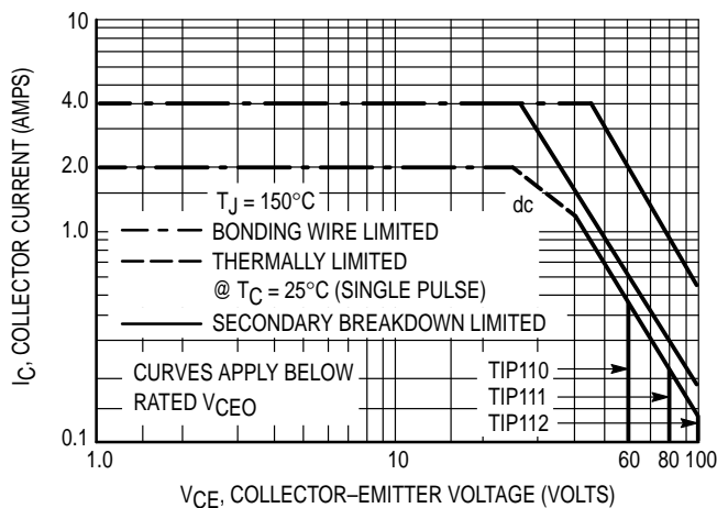
Figure 6. TIP110, 111, 112
