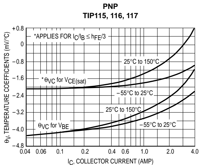
Figure 11. Temperature Coefficients
