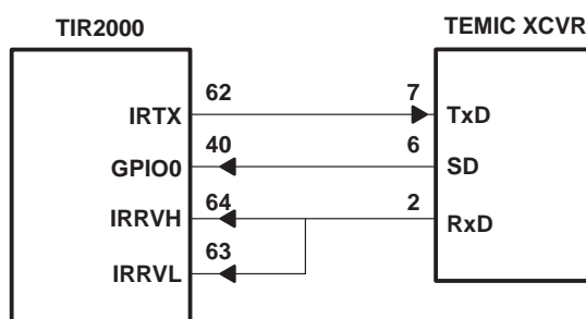
Figure 6–3. Temic Transceivers
