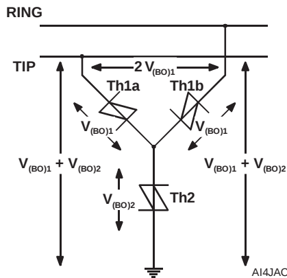
Figure 11. Protection Voltage
