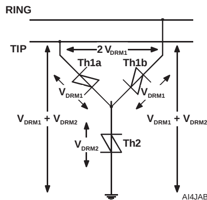
Figure 12. Off-State Voltage
