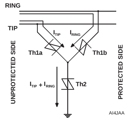
Figure 13. Current Flow
