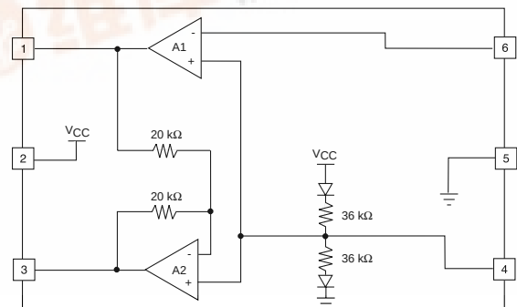
BLOCK DIAGRAM
