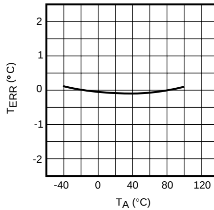
LINEARITY ERROR vs. TEMPERATURE
