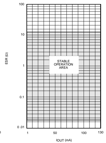
C_L = 10 \mu\text{F}
