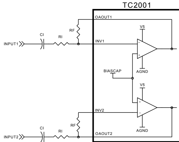
Figure 2: Input Stage
