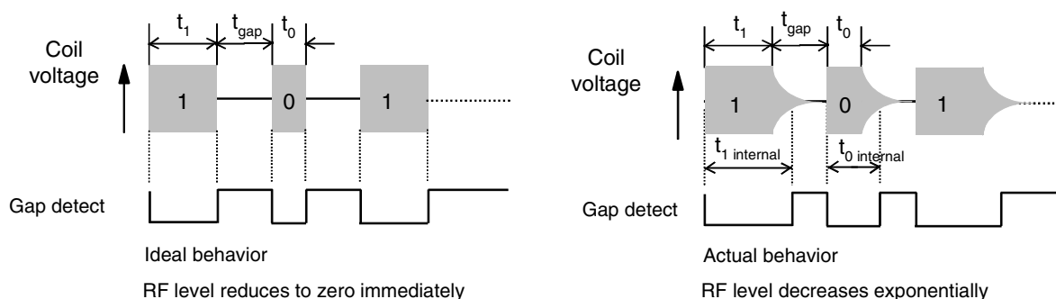
Figure 10. Ideal and Real Behavior Signals
