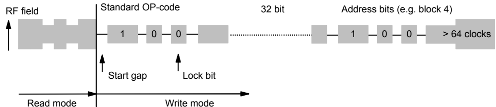
Figure 8. Write Protocol
