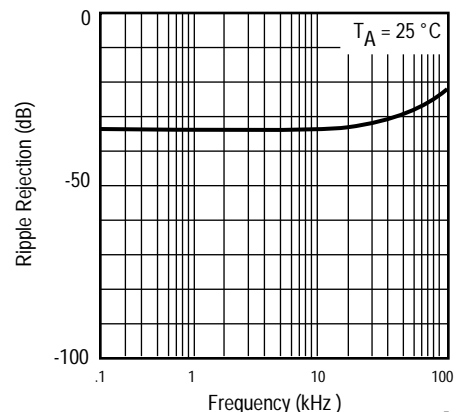
RIPPLE REJECTION
