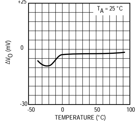
OUTPUT VOLTAGE DRIFT vs. TEMPERATURE
