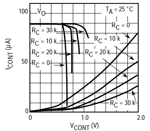
ON/OFF CONTROL TERMINAL (SERIES RESISTOR R_C)
