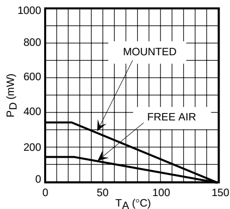
SOT-25 POWER DISSIPATION CURVE
