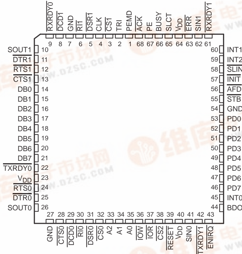
HV or FN PACKAGE (TOP VIEW)
