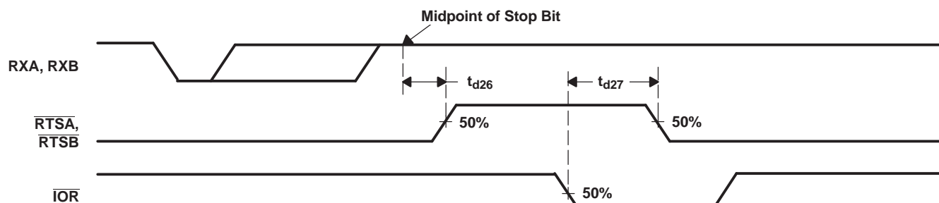
Figure 23. Auto- \overline{\text{RTS}} Timing for RCV Threshold of 1, 4, or 8 Waveforms
