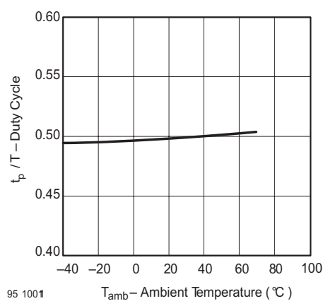
Figure 10. Duty Cycle vs. Ambient Temperature
