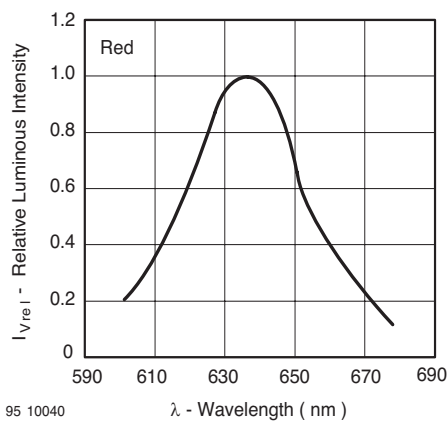
Figure 9. Relative Intensity vs. Wavelength
