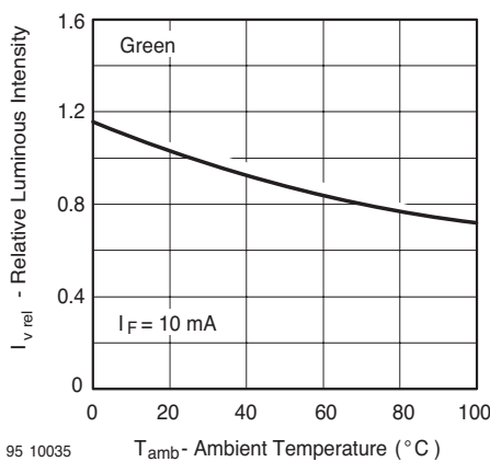
Figure 21. Rel. Luminous Intensity vs. Ambient Temperature
