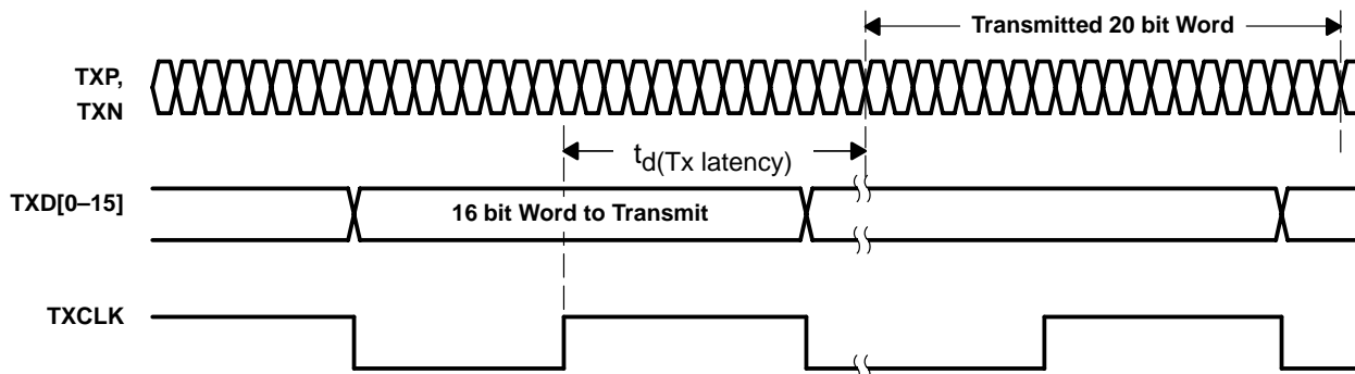
Figure 3. Transmitter Latency
