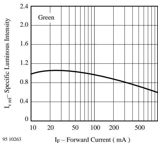
95 10263 Figure 22 Specific Luminous Intensity vs. Forward Current
