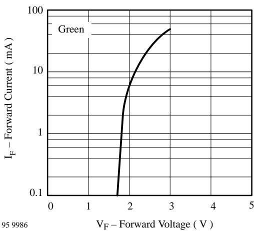
95 9986 Figure 20 Forward Current vs. Forward Voltage
