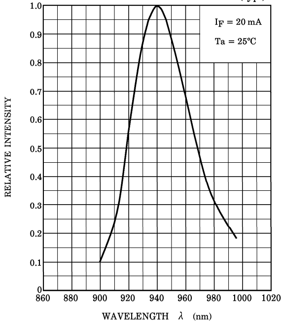
WAVELENGTH CHARACTERISTIC (typ.)
