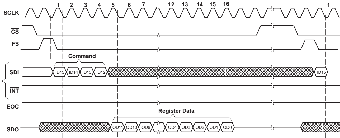
Figure 2. TLV1504/TLV1508 Read CFR Cycle (FS active)
