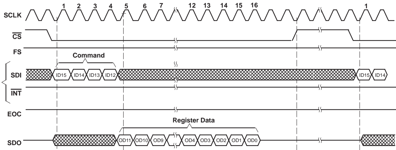
Figure 3. TLV1504/TLV1508 Read CFR Cycle (FS = 1)
