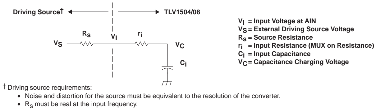
Figure 40. Equivalent Input Circuit Including the Driving Source
