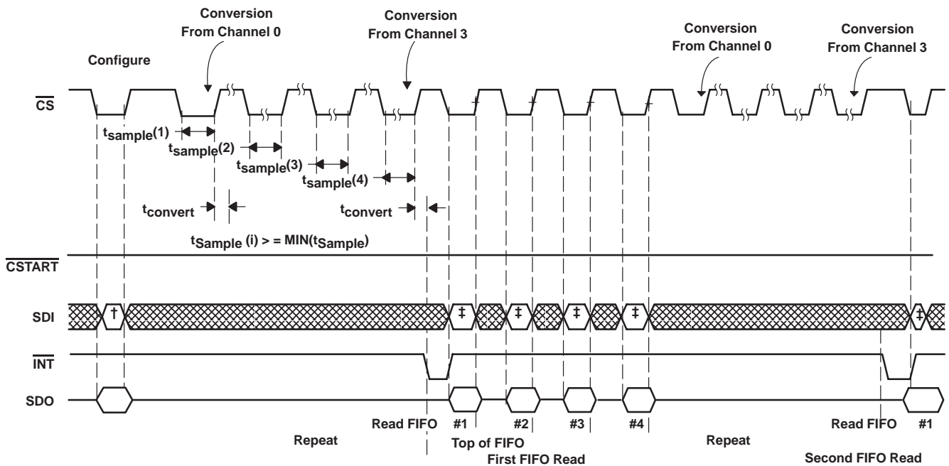
Figure 14. TLV1504/TLV1508 Mode 10/11 \mu p Serial Interface (Conversions triggered by CS)
