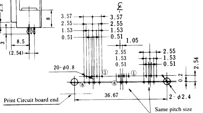
PCB mounting hole layout (Connector mounting side)
