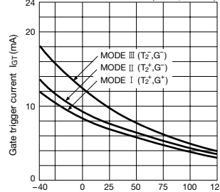
I_{GT} temperature characteristics (Typical)
